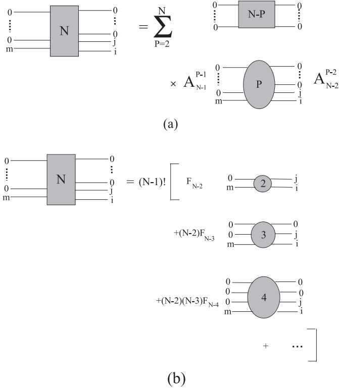
Fig. 15. Expansion of \langle v|B_0^{N-1}B_mB_i^\dagger B_j^\dagger B_0^{\dagger N-2}|v\rangle in terms of \langle v|B_0^{N-P}B_0^{\dagger N-P}|v\rangle as given in (a), and in terms of F_{N-P} as given in (b), (see Eq. (32)). The way to go from (a) to (b) is the same as in Figure 5.
