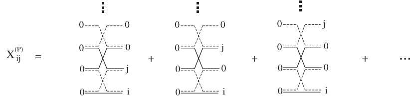
Fig. 9. Connected fermion exchanges between the cobosons (i, j) and P-2 cobosons 0 leading to P cobosons 0.
