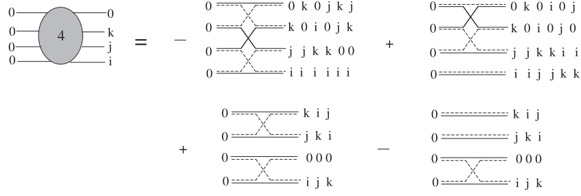
Fig. 12. Topologically different exchange processes between the cobosons (i, j, k) and one coboson 0 leading to 4 cobosons 0. The first two diagrams appear 6 times with different index positions, while the last two diagrams appear 3 times.
