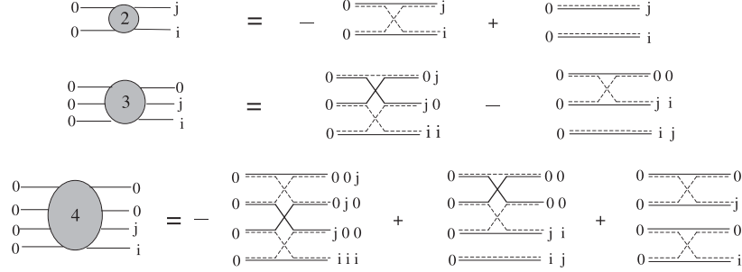
Fig. 10. Connected and disconnected fermion exchanges between the cobosons (i, j) and P-2 cobosons 0 leading to P cobosons 0, for P = 2, 3, 4 . Note that in these diagrams, the cobosons 0 are “never alone”, i.e., they are connected to i and/or j . The various columns of indices, which correspond to topologically different diagrams, have to be taken alternatively. So that the first diagram with P = 4 cobosons actually corresponds to 3 diagrams.
