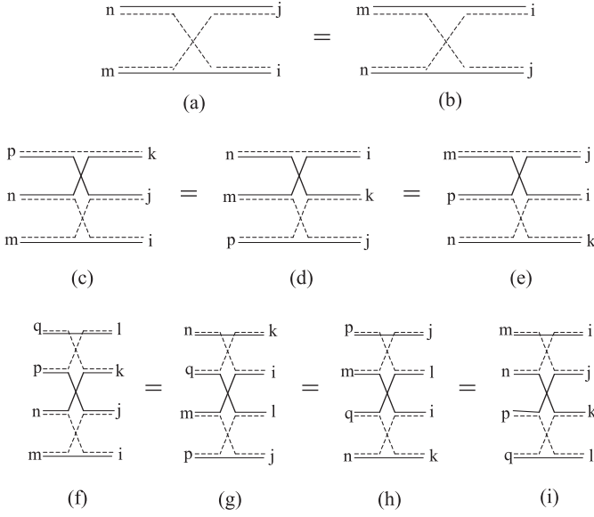
Fig. 3. (a,b): The two Shiva diagrams representing the fermion exchange between the two cobosons (i, j) , in which m and i have the same fermion \alpha . (c–e): The Shiva diagrams representing the fermion exchanges between the three cobosons (i, j, k) , in which (m, i) , (p, j) and (n, k) have the same fermion \alpha . (f–i): The four Shiva diagrams representing the fermion exchanges between the four cobosons (i, j, k, l) , in which (m, i) , (p, j) , (n, k) and (q, l) have the same fermion \alpha .
