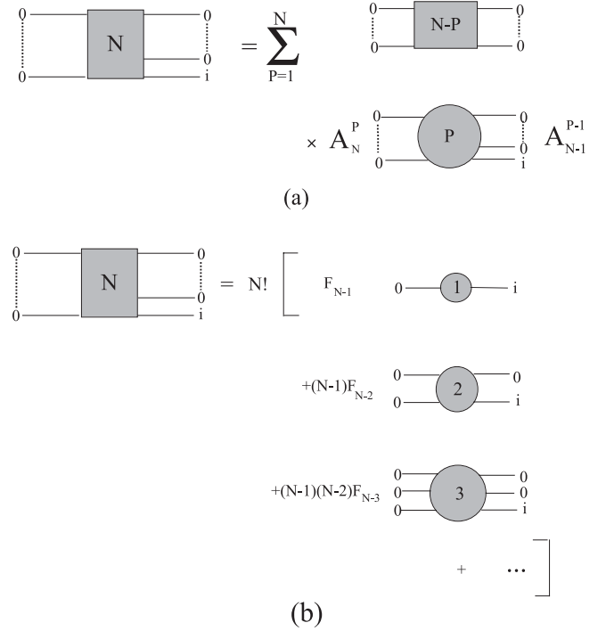
Fig. 5. Expansion of the scalar product \langle v | B_0^N B_i^\dagger B_0^{\dagger N-1} | v \rangle in terms of \langle v | B_0^{N-P} B_0^{\dagger N-P} | v \rangle , represented by the diagram with cobosons 0 only, as given in (a), and in terms of F_{N-P} as given in (b), (see Eq. (23)). To go from (a) to (b), we just use \langle v | B_0^{N-P} B_0^{\dagger N-P} | v \rangle = (N-P)! F_{N-P} and the value of A_N^P given in equation (22), which corresponds to the number of ways to choose the P cobosons 0 of the left, among N .
