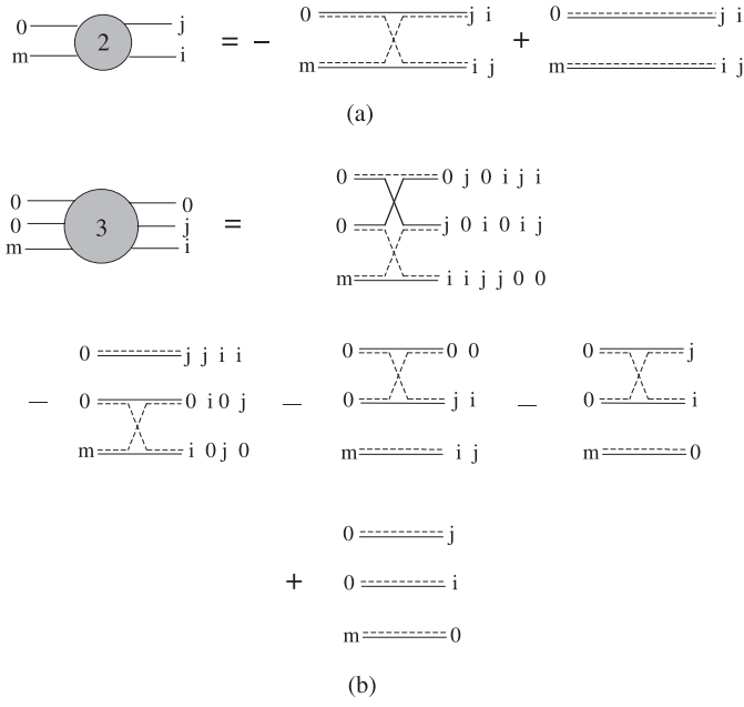
Fig. 16. Topologically different exchange processes, connected or not, between the cobosons (i, j) and (P - 2) cobosons 0, giving the coboson m and (P - 1) cobosons 0, for P = 2, 3 . The first diagram of (b) appears 6 times, which corresponds to all the possible positions of (i, j) in this Shiva diagram. And so on.
