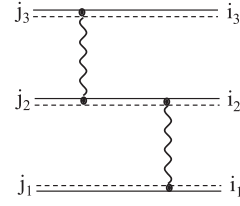
Fig. 1. A possible direct interaction between three cobosons, starting in states (i_1, i_2, i_3) and ending in states (j_1, j_2, j_3) . As in all the diagrams of this paper, the fermions \alpha are represented by solid lines and the fermions \beta by dashed lines.
