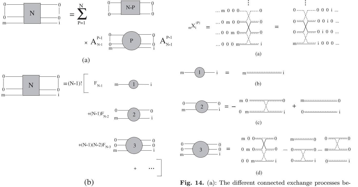
Fig. 13. Expansion of \langle v|B_0^{N-1}B_mB_i^\dagger B_0^{\dagger N-1}|v\rangle in terms of \langle v|B_0^{N-P}B_0^{\dagger N-P}|v\rangle as given in (a), and in terms of F_{N-P} as given in (b), (see Eq. (29)). The way to go from (a) to (b) is the same as in Figure 5.
