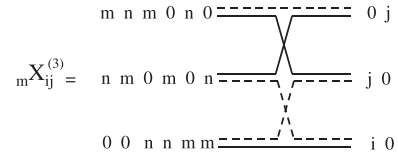
Fig. 18. The connected exchange process between the cobosons (i, j, 0) giving the cobosons (m, n, 0) . This Shiva diagram appears (6 \times 2) times, due to the topologically different positions of the various indices.
