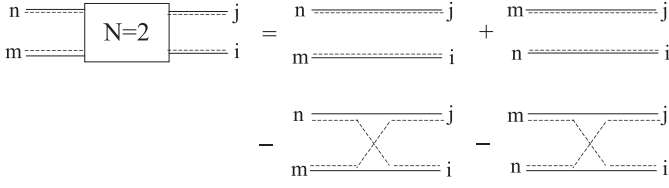
Fig. 2. Scalar product of two cobosons given in equation (12). It contains two sets of \delta terms which correspond to the two upper diagrams. These \delta terms exist for elementary bosons. This two-coboson scalar product also contains two exchange terms which are missed when cobosons are replaced by elementary bosons. Note that these two exchange diagrams are related by a (m \leftrightarrow n) permutation which is equivalent to a (i \leftrightarrow j) permutation.
