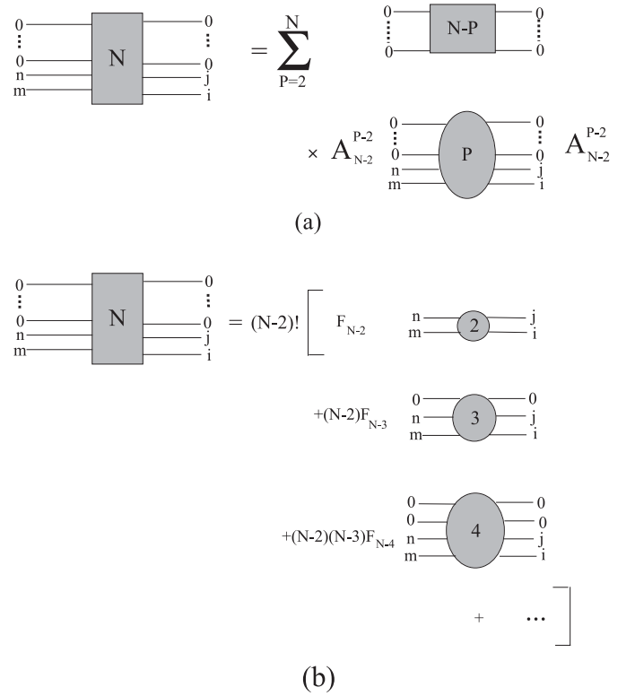
Fig. 17. Expansion of \langle v | B_0^{N-2} B_m B_n B_i^\dagger B_j^\dagger B_0^{\dagger N-2} | v \rangle in terms of \langle v | B_0^{N-P} B_0^{\dagger N-P} | v \rangle as given in (a), and in terms of F_{N-P} as given in (b), (see Eq. (35)). The way to go from (a) to (b) is the same as in Figure 5.
