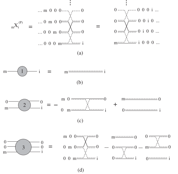
Fig. 14. (a): The different connected exchange processes between the coboson i and (P - 1) cobosons 0, leading to the coboson m and (P - 1) cobosons 0. (b–d): Topologically different exchange processes, connected or not, between the coboson i and (P - 1) cobosons 0 leading to the coboson m and (P - 1) cobosons 0, with P = 1, 2, 3 . The first diagram of (d) appears 3 times.
