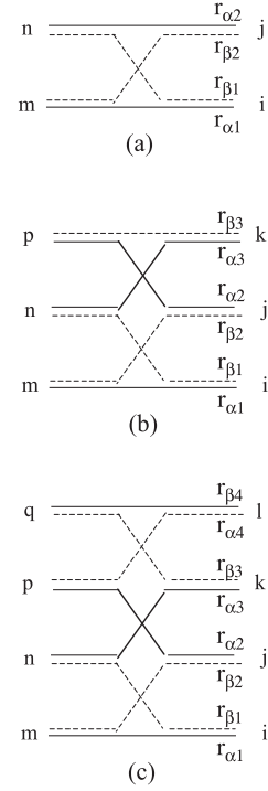
Fig. 4. Shiva diagrams between 2, 3 and 4 cobosons corresponding to the integrals given in equations (11, 18, 20).
