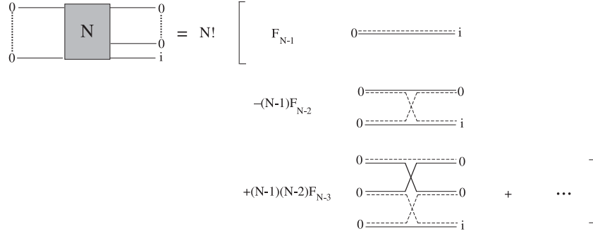
Fig. 7. Expansion of \langle v|B_0^N B_i^\dagger B_0^{\dagger N-1}|v\rangle in Shiva diagrams.
