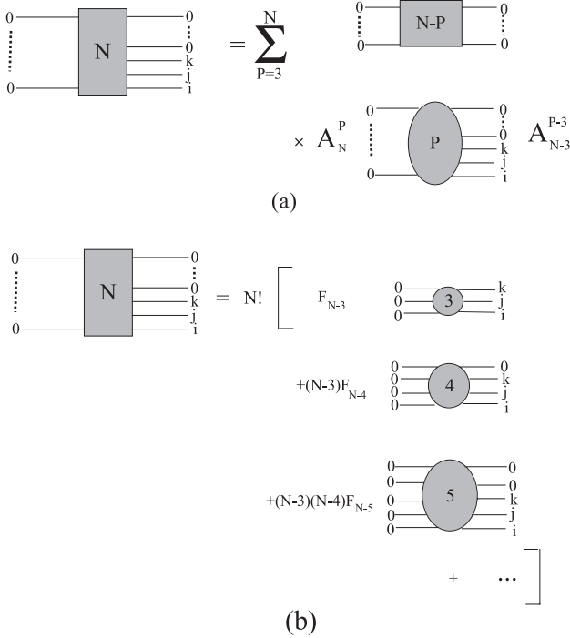
Fig. 11. Expansion of \langle v|B_0^N B_i^\dagger B_j^\dagger B_k^\dagger B_0^{\dagger N-3}|v\rangle in terms of \langle v|B_0^{N-P} B_0^{\dagger N-P}|v\rangle as given in (a), and in terms of F_{N-P} as given in (b). The way to go from (a) to (b) is the same as in Figure 5.
