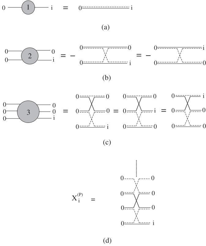
Fig. 6. (a–c): Fermion exchanges between the coboson i and (P-1) cobosons 0 , for P = 1, 2, 3 respectively. (d): The factor X_i^{(P)} defined in equation (24), which corresponds to the Shiva diagram with P cobosons 0 on the left and the coboson i plus (P-1) cobosons 0 on the right.
